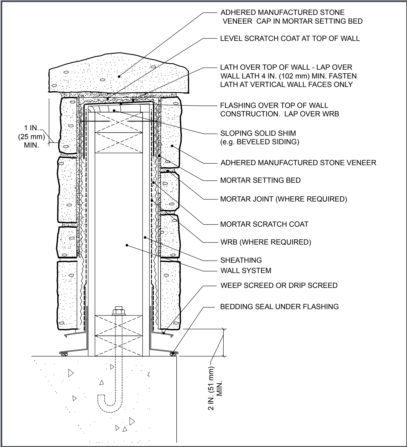
Figure 34. Wall Cap
