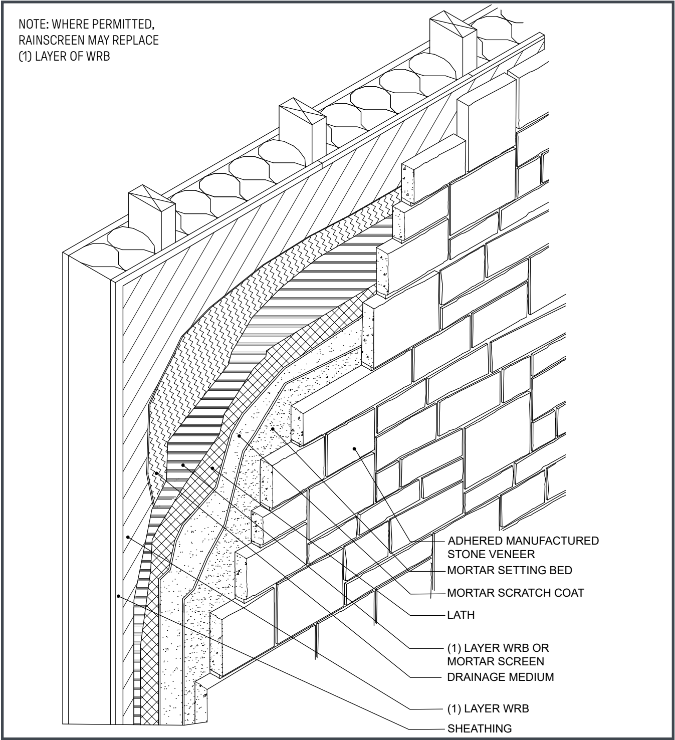
Figure 35. Wall Assembly – Rainscreen System – Membrane System
