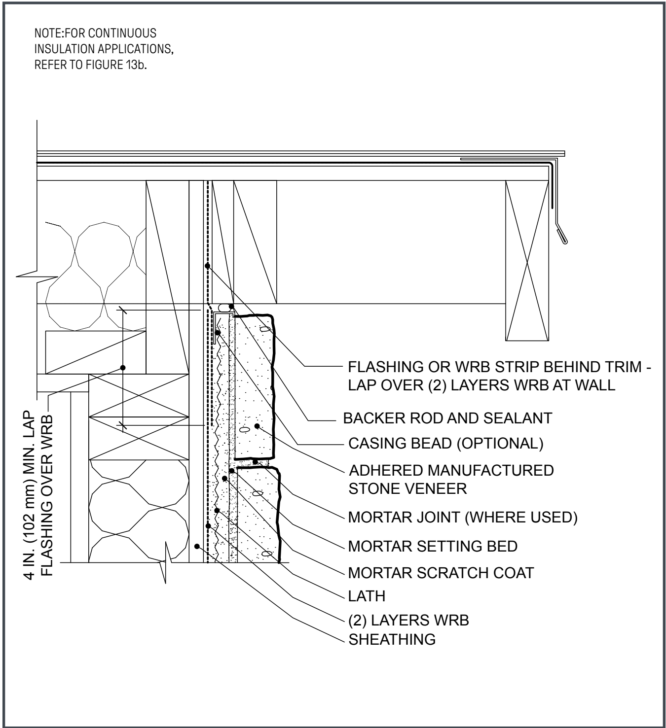
Figure 15. Rake - Overhang
