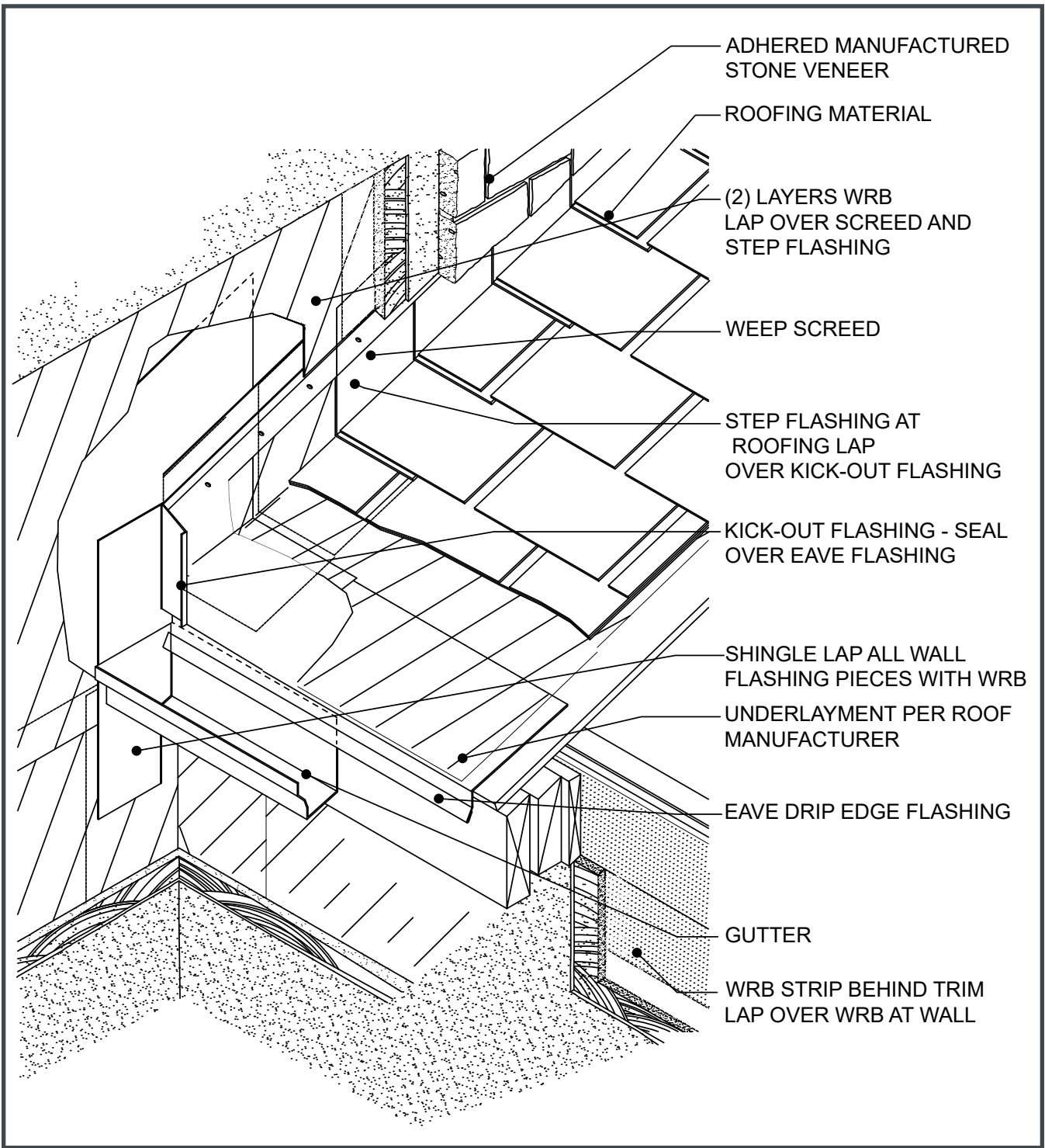
Figure 24. Kick-Out Flashing
