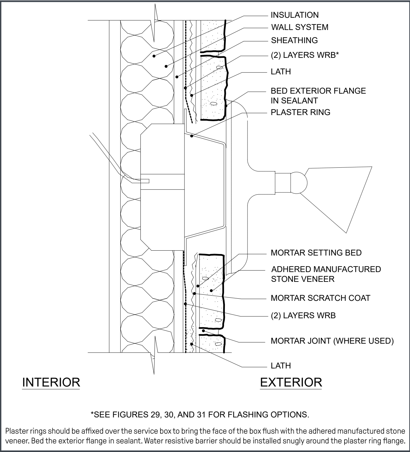
Figure 31. Penetration, Fixture
