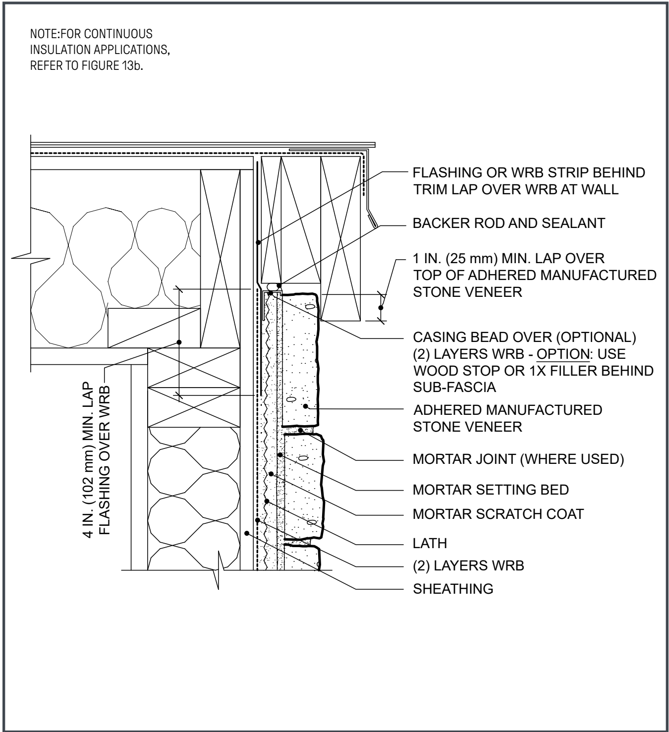
Figure 16. Rake - Flush
