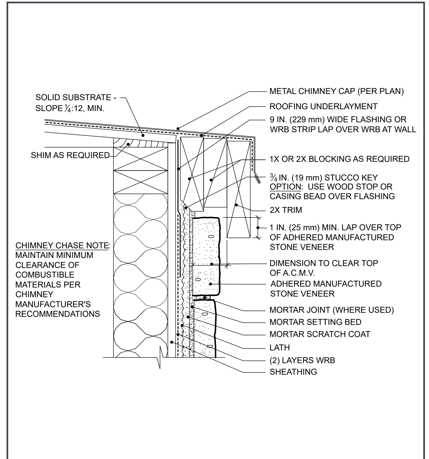
Figure 26. Chimney Chase
