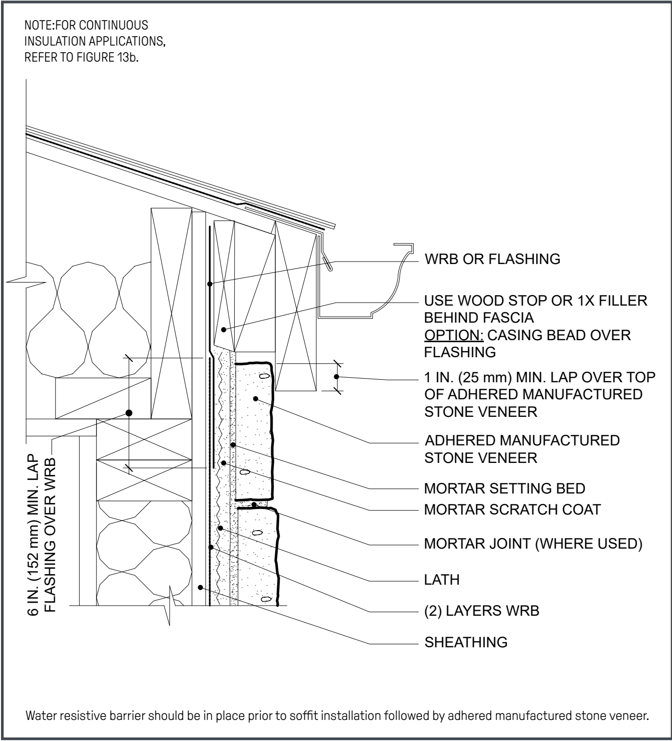
Figure 14. Open Eave - Flush
