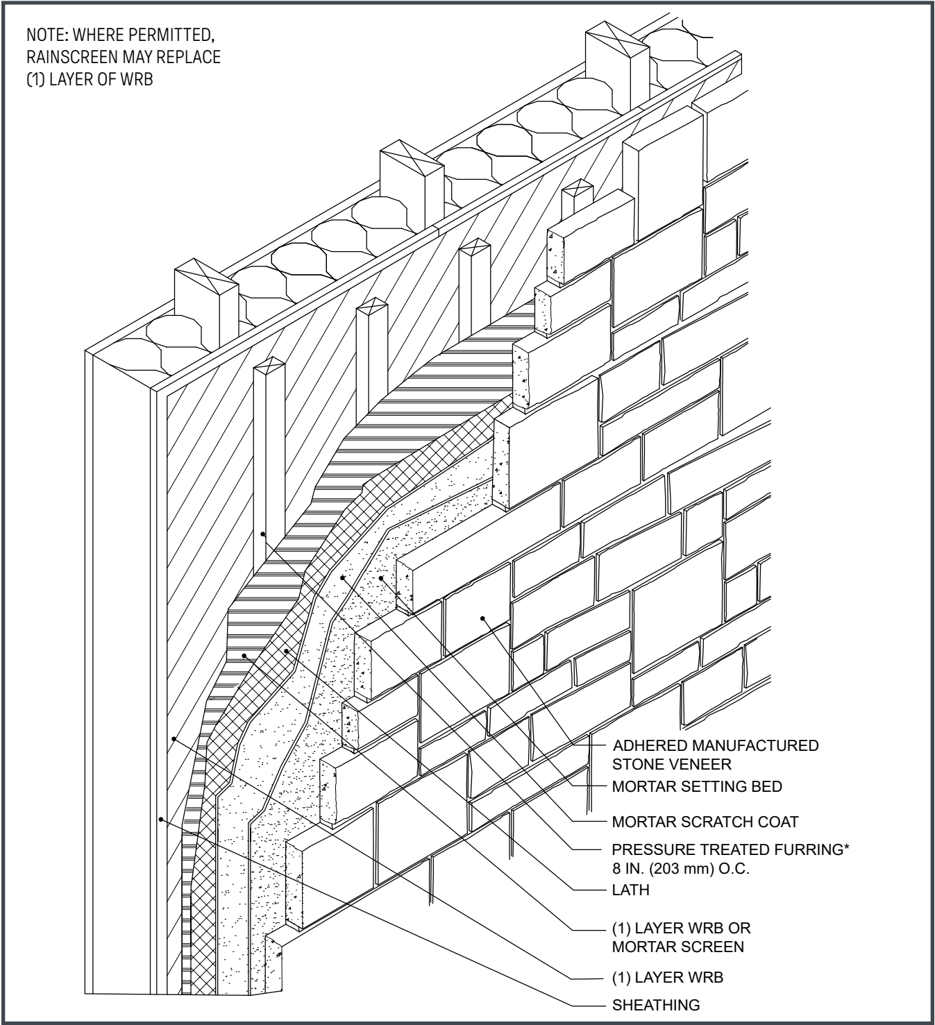
Figure 36. Wall Assembly – Rainscreen System – Strapped
