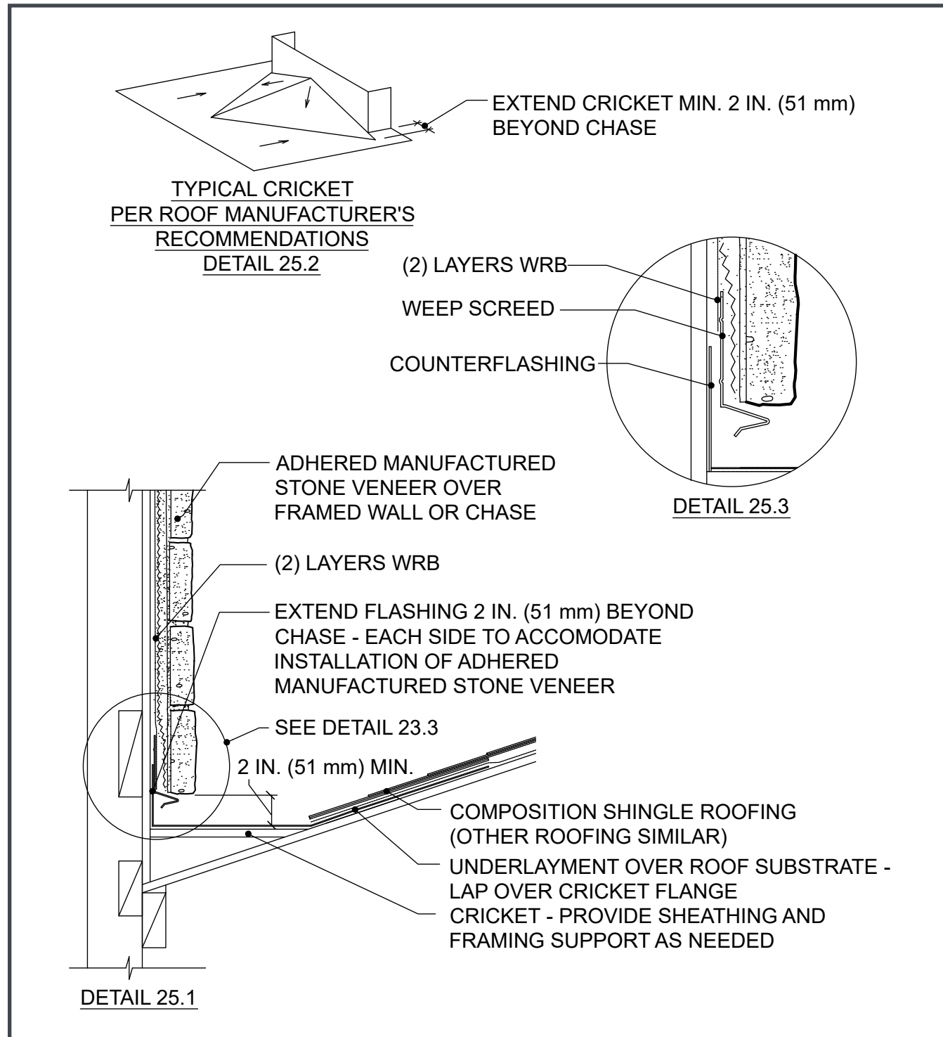
Figure 25. Cricket
