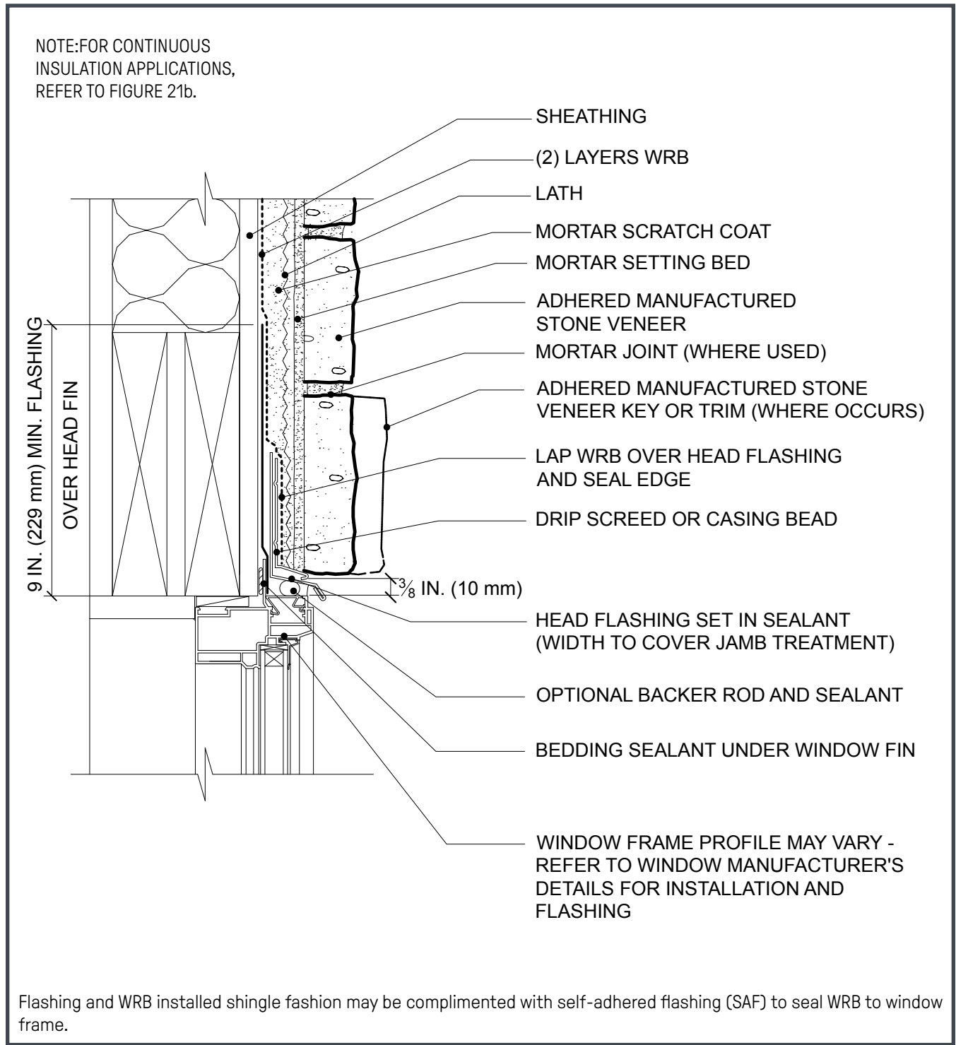
Figure 23. Window Head
