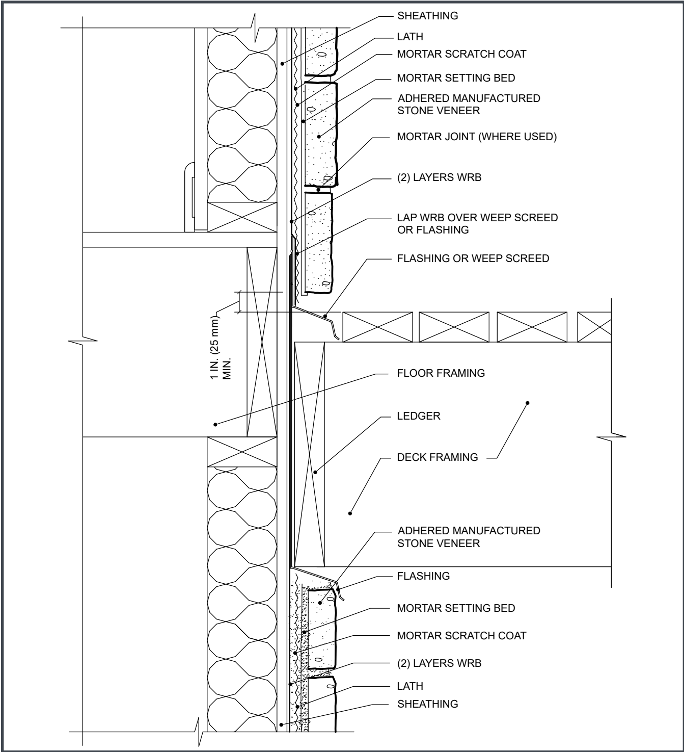
Figure 33. Deck Termination
