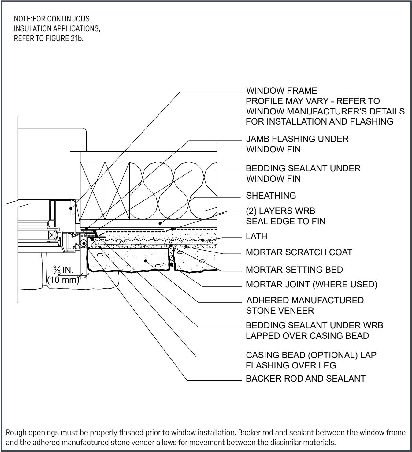
Figure 22. Window Jamb
