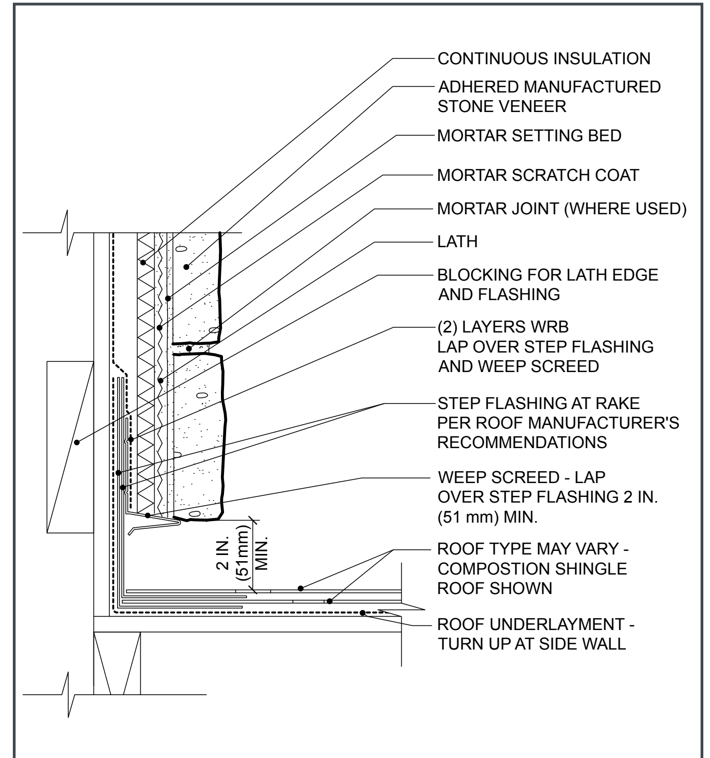
Figure 17b. Side Wall – Composition Shingles Over Continuous Insulation
